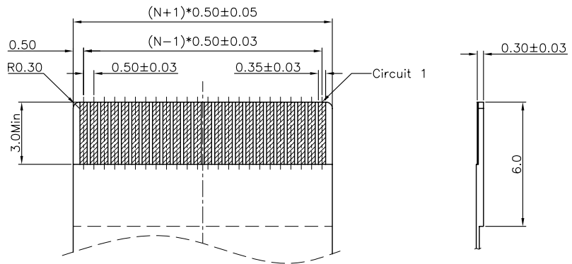
RECOMMENDED FPC/FPC DIMENSION
